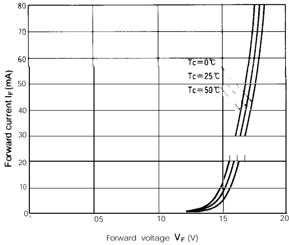
Fig. 83-1 Forward Current vs. Forward Voltage
