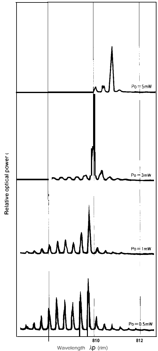
Fig. 83-5 Optical Power Output Dependence of Wavelength
