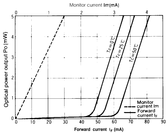
Fig. 83-2 Optical Power Output vs. Forward Current and Monitor Current
