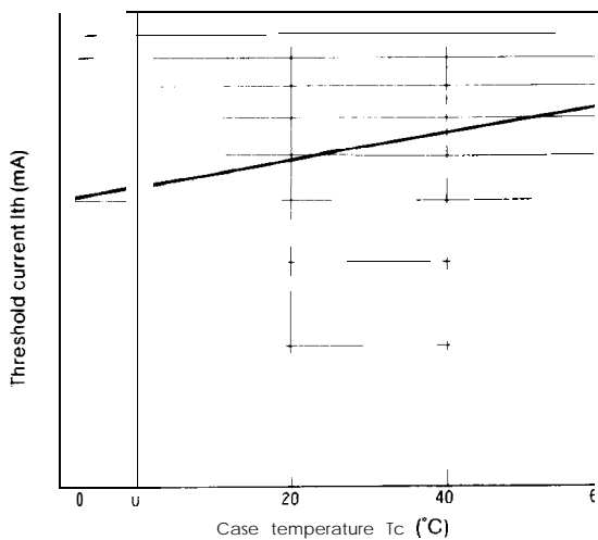
Fig. 83-3 Threshold Current vs. Temperature
